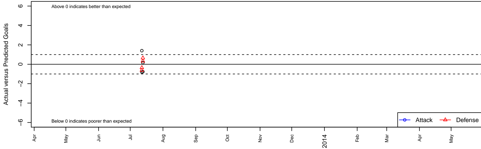
Washington Timbers Red – Unk B95 Dots are actual minus expected GF (blue circles) and GA (red triangles). Blue line is smoothed change in attack strength. Red is smoothed change in defense strength.
